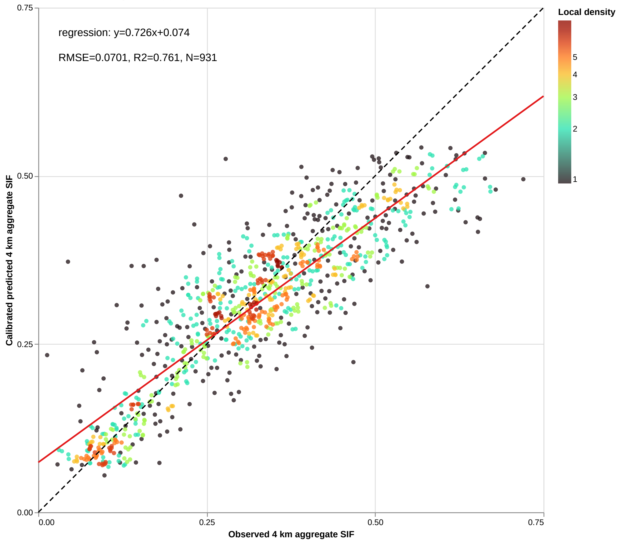
4 km Spatial-Aggregate U-Net: Observed vs. Predicted SIF, Test RMSE=0.0701, R2=0.761
